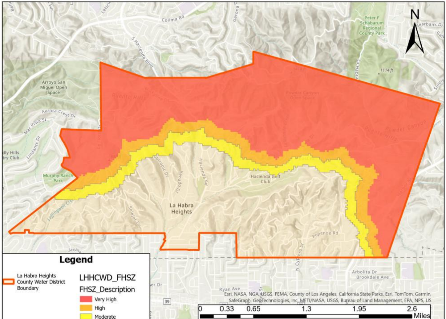
Figure 3. Wildfire Map with LHHCWD Boundaries La Habra Heights County Water District: Fire Hazard Severity
